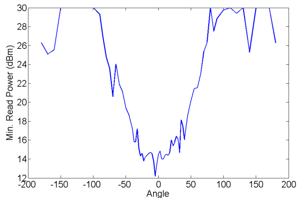
Fig. 7: Far-field measured minimum power to read tag 2.13m away, versus bearing to tag
